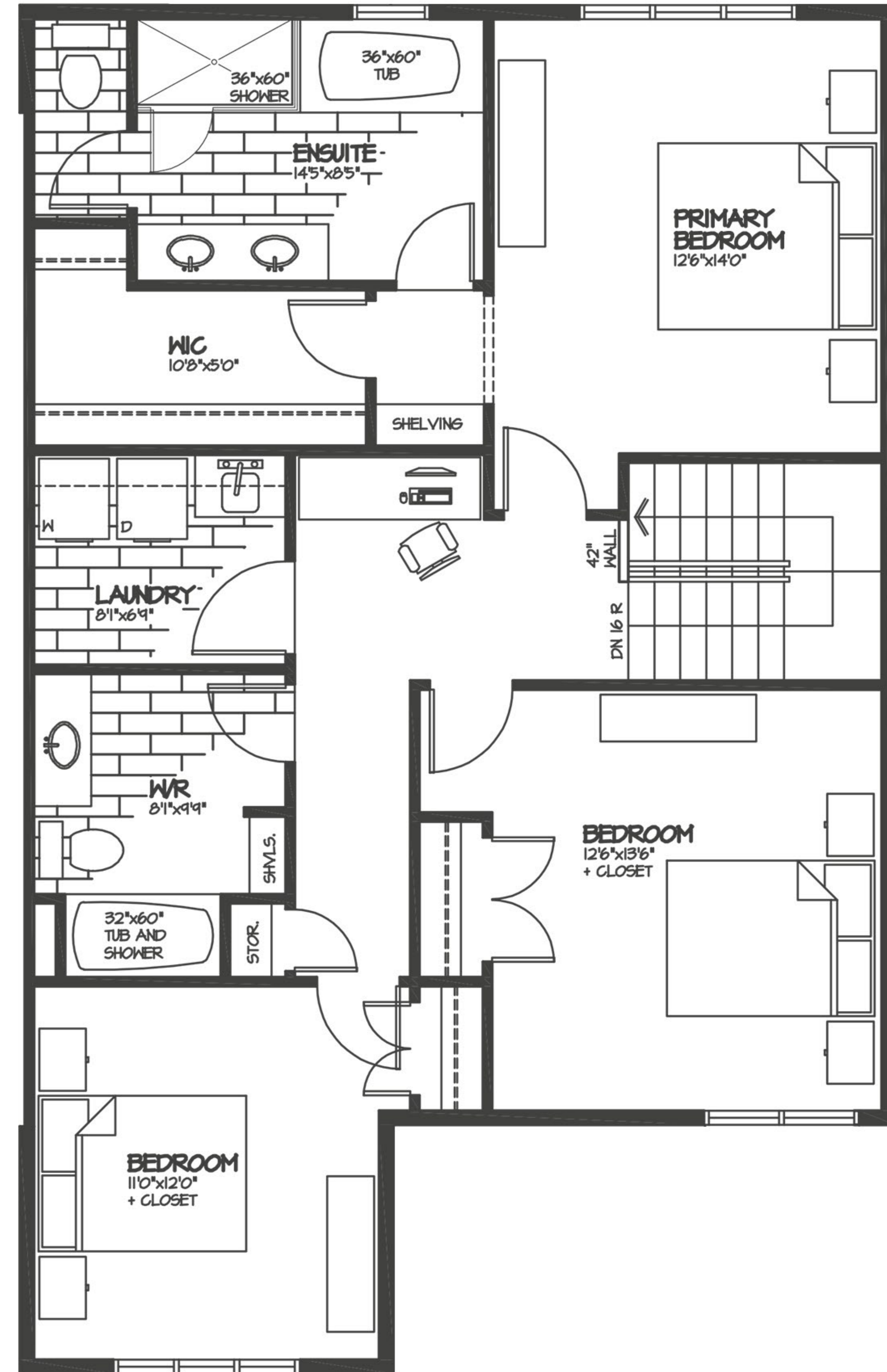
Upper Floor 1042 sq. ft.
