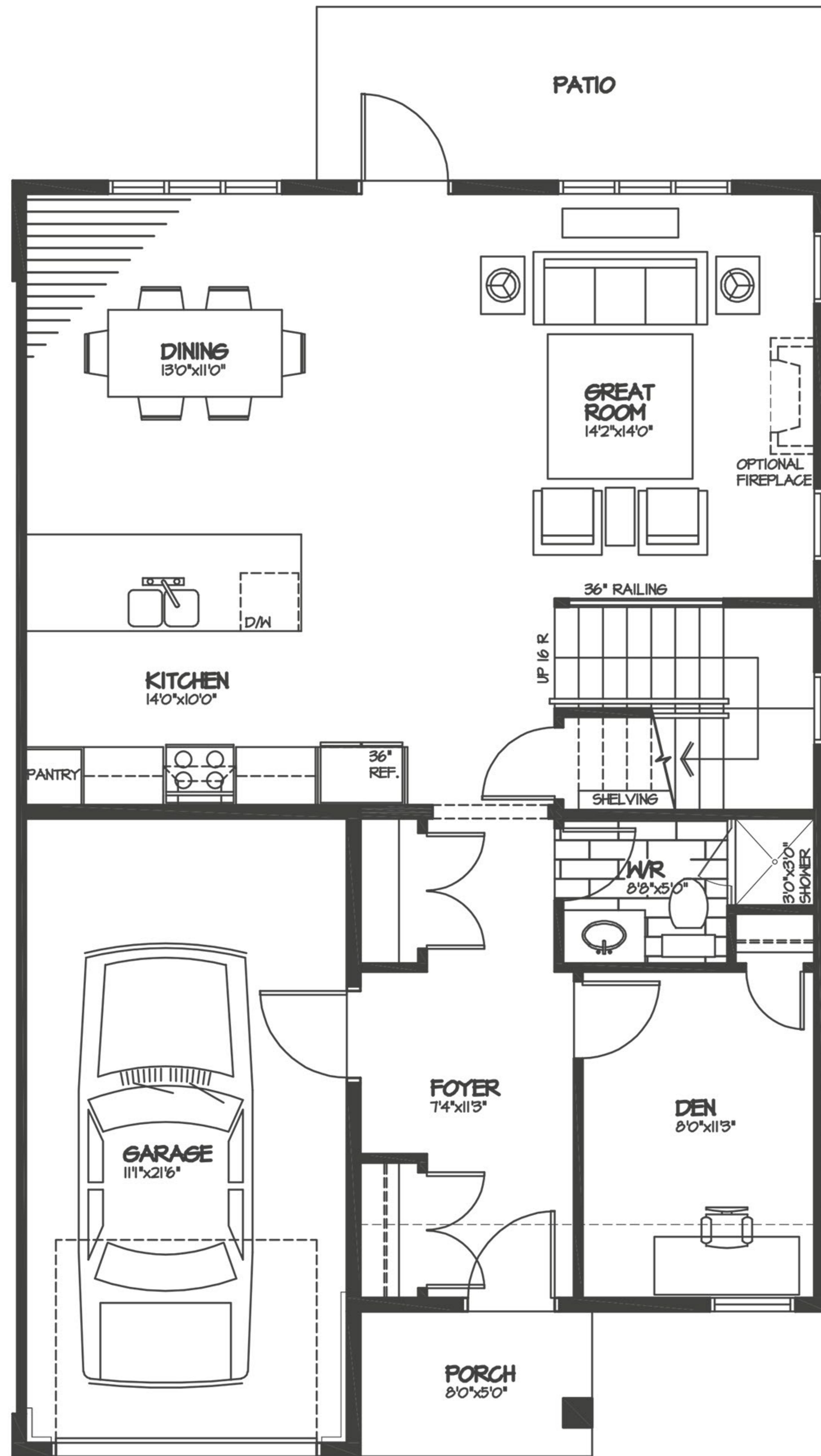
Main Floor 898 sq. ft.
